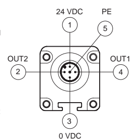
Receiver M12 5-pole
